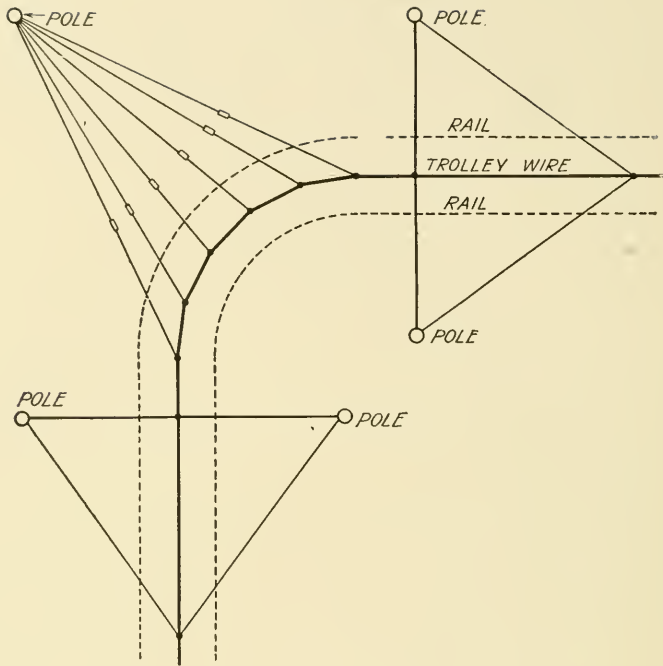
Fig. 192. Line Construction on a Curve Using Five Poles
